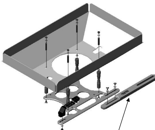
Throttle Stop Bracket #555-55016 (Not Included), Installed as shown.
