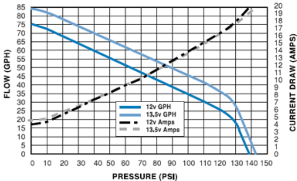
Flow vs. Pressure @ 12 and 13.5 VDC in Stoddard Solvent
