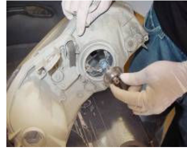
Step 12: Remove the headlight bulb.
