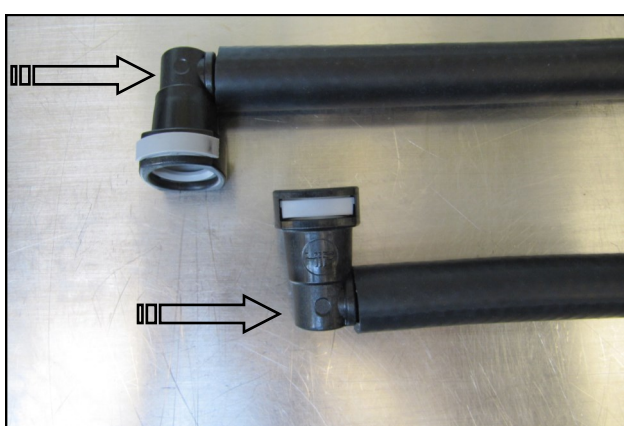
7. Insert the new Quick Connect Fittings into the supplied Breather Hoses.
