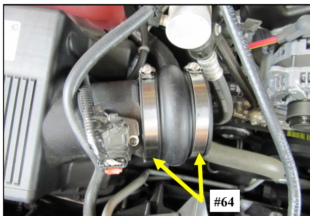
5. Slide the Hump Hose and two #64 Clamps onto the factory air box. If you are installing an Airaid Jr. kit, install the Airaid Premium Filter at this time.
