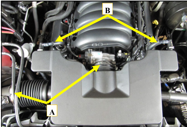
1. Disconnect The Negative Battery Terminal! A.) loosen the clamps securing the intake system to the throttle body and the air box. B.) Disconnect the valve cover breathers from either side of the factory intake System. Remove the factory intake system and set it aside.
