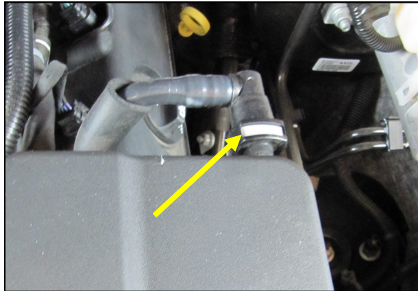
2. The quick connects for the valve cover breathers are removed by depressing the grey locking tab in the fitting and sliding them off.
