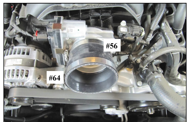
6. Slide the Reducer and the #56 and 64 clamps onto the throttle body.
