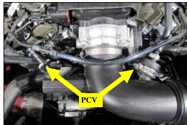
3. Disconnect the PCV breather lines from the intake tube.
