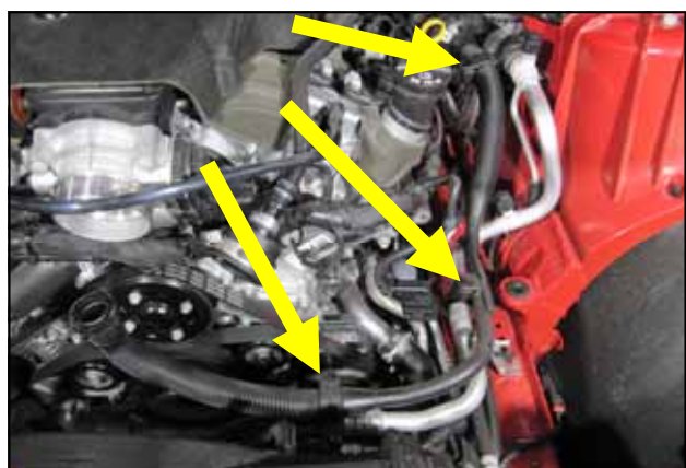
7. Disconnect the resonator tube retainers on the along A/C line, all the way up to the strut tower.
