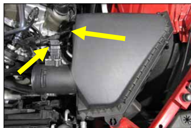
6. Disconnect the Mass Airflow sensor and gently pry the harness anchor out of the airbox. Remove the airbox assembly from the vehicle. Ensure that all three airbox grommets remain in the inner fender and not on the airbox.
