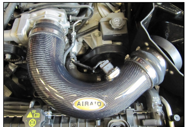
17. Install the Airaid Intake Tube (#2) into the Hump Hose first, and then into the reducing coupler. Adjust for fit, and tighten all four Hose Camps. It is Very important to verify that the Intake Tube is not rubbing on the Radiator or the hood.
