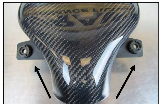
9. Transfer the factory intake tube mounting grommets into the Tube Brackets as shown.
