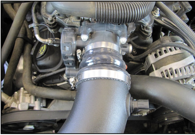
13. Open and Install the Clamps onto the Coupler as shown with the #44 clamp on the throttle body (#9) and the #52 clamp (#8) on the Intake Tube.
