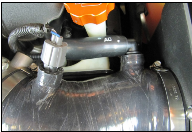
10. Reconnect the air temperature sensor, and the crankcase breather tube to the Barbed Elbow .
