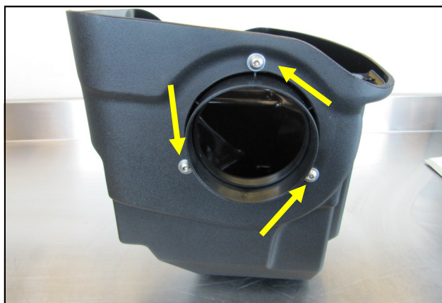
4. Install the Filter Adapter onto the Cool Air Box using the three 1/4" Button Head Screws and 1/4" Flat Washers.
