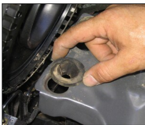
6. Remove the two factory grommets from the body and discard.
