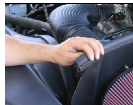
12. Install the supplied weather strip on the top edge of the Airaid Cool Air Dam. Note: The weather strip is pre cut to the proper length. Start from one end and work your way around to the other end to insure even placement.
