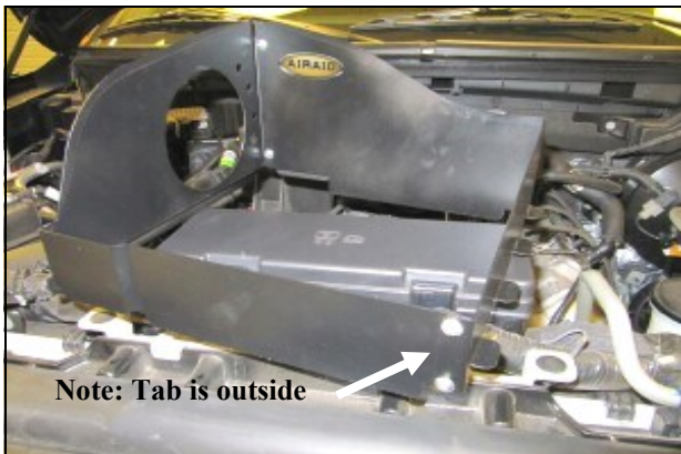
4. Assemble the two Quick Fit panels (#3 & #4) as shown using four 6-32 screws (#7) flat washers (#9) and kep nuts (#8). Note: Tab is outside
