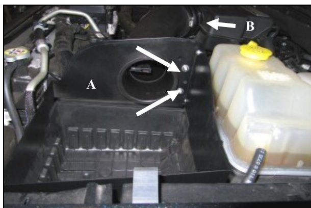
8. A.) Mount the Intake Tube to the Rear Panel using the two 1/4-20 Button Head Bolts (#11) and 1/4" Flat washers (#12). B.) Slide the Hump Hose and clamps onto the engine air inlet, check for alignment, and tighten the clamps.
