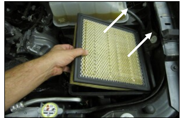
3. Remove the factory air filter from the lower half of the airbox.
