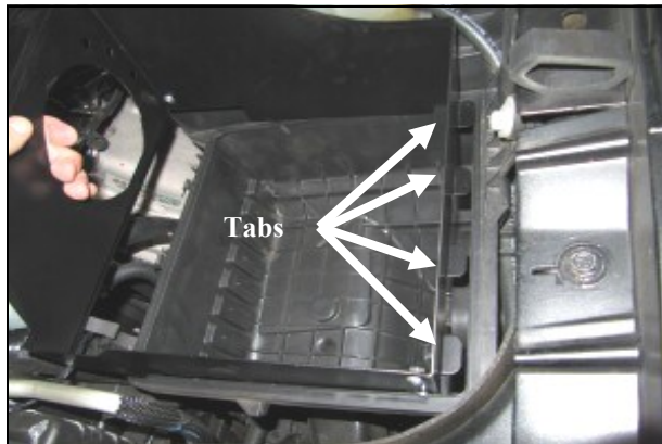
5. Install the assembly onto the lower half of the factory airbox. Slide the metal tabs into the airbox slots, and fasten the 3 airbox clips.
