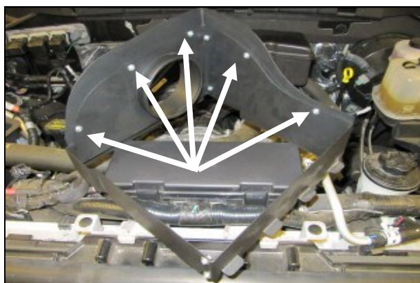
5. For F-150 models only: Fasten the Extension panel (#5) to the outside of the panel assembly using the remaining 6-32 screws, flat washers, and keps nuts.
