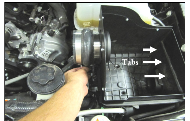
6. A.) Install the Silicone Hump Hose (#7) and two #64 Hose Clamps (#14) onto the Quick Fit assembly. Leave the clamps loose for now. B.) Install the assembly onto the lower half of the factory airbox. Slide the metal tabs into the airbox slots, and fasten the 3 airbox clips.
