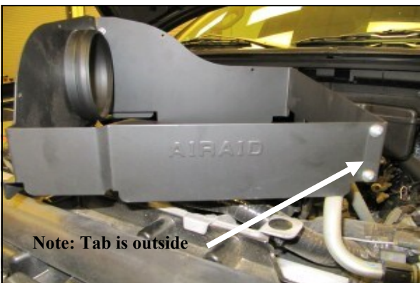
4. Assemble the two Quick Fit panels (#3 & #4) as shown using four 6-32 screws (#9) flat washers (#11) and keps nuts (#10). Note: Tab is outside
