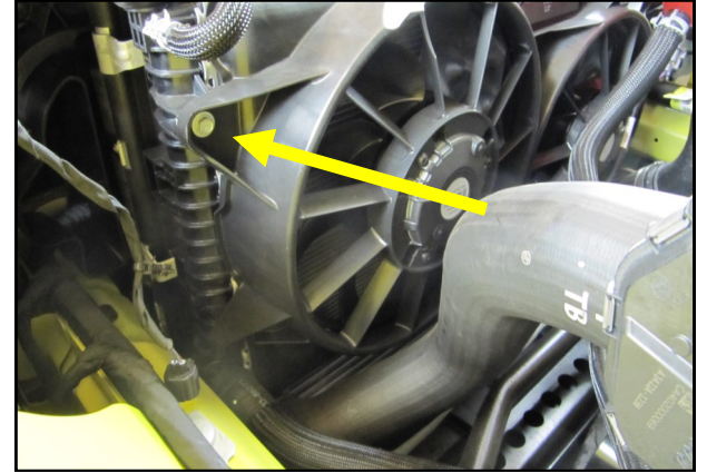
10. Remove the drivers side fan shroud bolt and set it aside.
