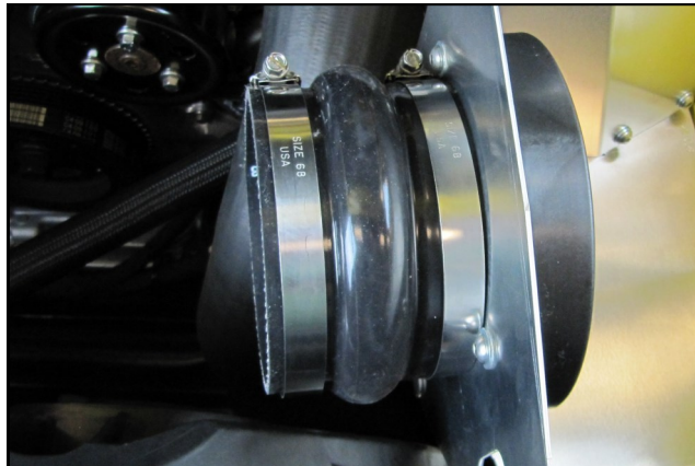
11. Slide the Hump Hose with two, #68 Clamps onto the Filter Adapter .
