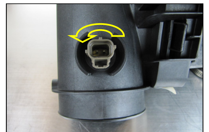
8. Tilt the air temp sensor rearward so the locking tab clears the ramp and rotate it counterclockwise 1/4 turn to release it.
