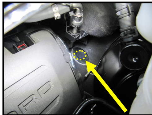
20. Reconnect air flow meter and plug the wire harness anchor into the Airbox wall.
