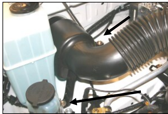
2. With a 12mm socket, remove two bolts that hold the intake tube to the fender.
