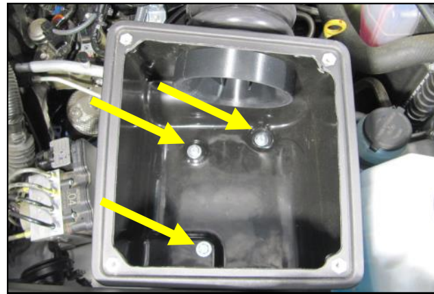
17. Mount the Airaid Airbox onto the CAB Mounts using the three 8mm Bolts and 5/16 Flat Washers
