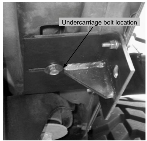
Front Bracket Installed (bracket #2)
