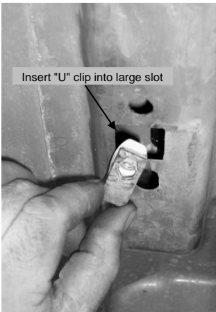
Insertion of "U" clip Photo Group 1
