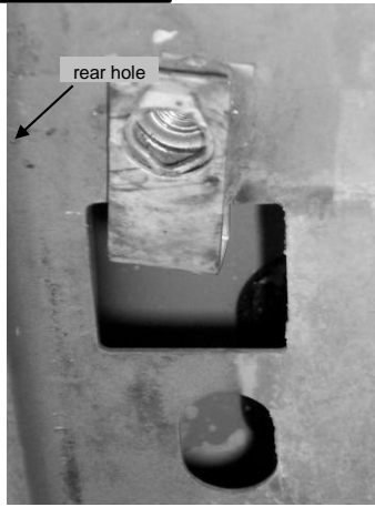
"U" clip Installed
