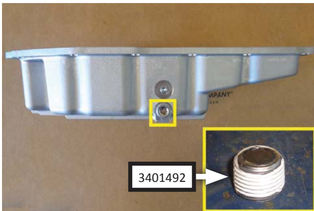
12. Apply Teflon tape to socket plug (3401492) before installing it into deep pan.
