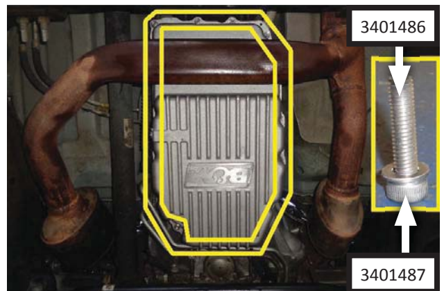
16. Install deep pan with 25MM screws (x15) (3401486) and flat washers (x15) (3401487) hand-tight. Then torque screws to 8ft lbs.
