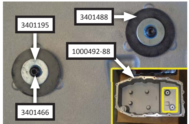
10. Apply loktite onto threads of 10mm screws (x2) (3401466) then install them through lock washers (x2) (3401195) and oversized flat washers (x2) (3401488) into deep pan (1000492-88) to secure factory magnets.
