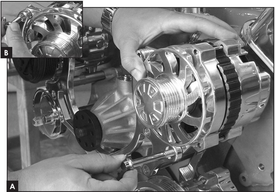
Figure 10: Attaching Alternator
