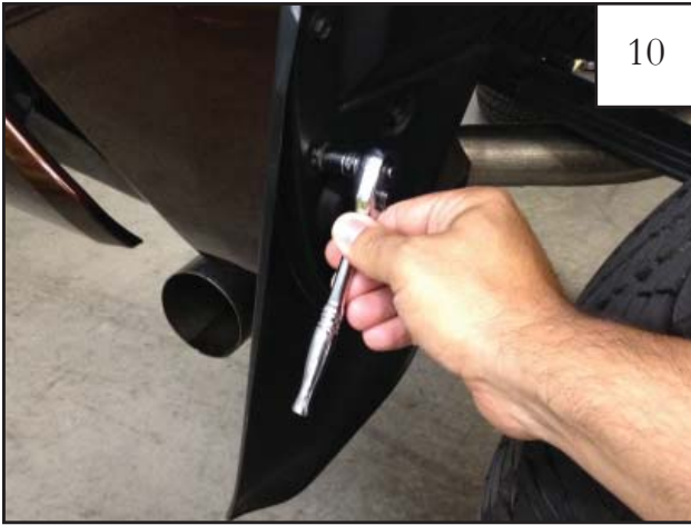
Using a socket wrench with a 10mm socket, factory screw second from the top of the mud guard.
