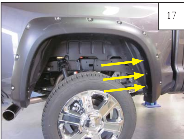
Using 10mm socket, start three supplied 20mm Hex Screws through the forward most holes of flare and into factory holes in fender.
