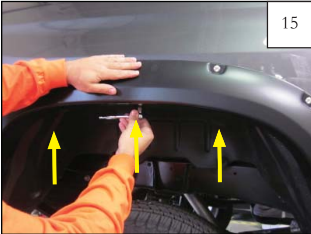
Hold the flare firmly on the fender. Start three supplied 20mm Hex Screws (SW1-0036) through the top center holes of the flare and into factory holes in fender.
