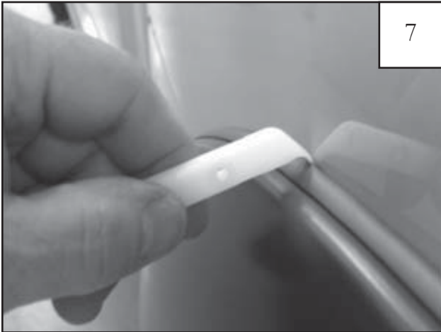
7 Using supplied Edge Trim Tool (ET1-0002), seat edge trim against vehicle by hooking curved end under edge trim at one end of flare. Next, slide around outer edge of flare to the other end.
