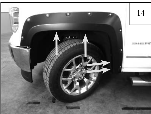
Press and hold Flare on vehicle, install supplied screw (SW1-0056) into the two upper and lower factory holes locations. Do not fully tighten at this time.
