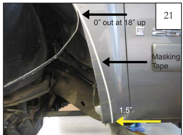
21 At the bottom of cut fender, measure 1.5" toward door seam and make a mark. Use masking tape to created a reference line from mark at bottom up to the 18" point.
