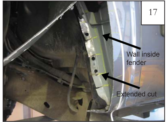
17 After bending flange of inner fender support straight, make the cuts go further to meet with the wall inside the fender.
