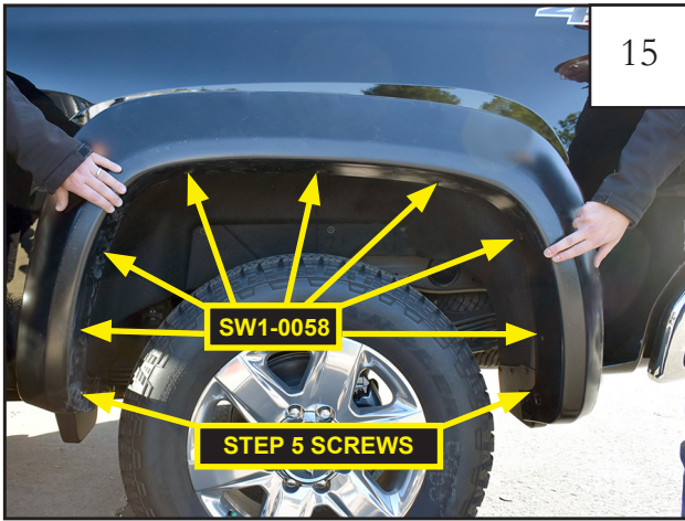
15 Install rear flare using (7) SW1-0058 truss screws and the (2) outboard screws removed in Step 9.
