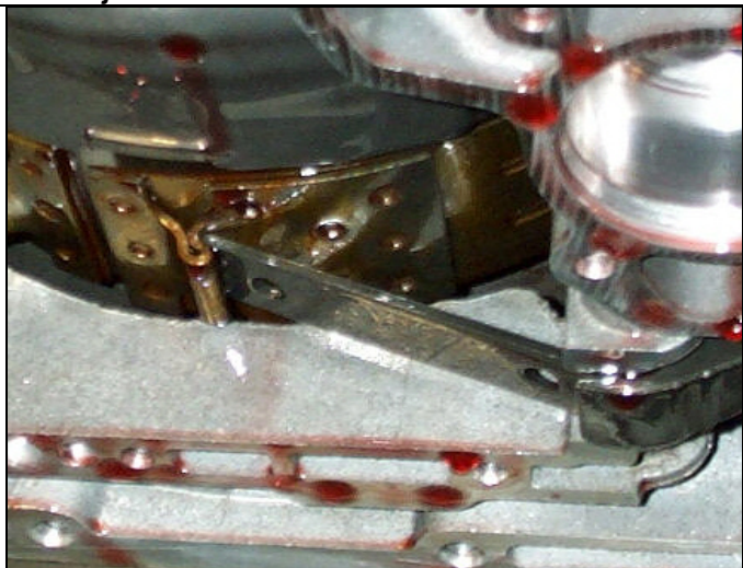
Stock Band Strut in Place
