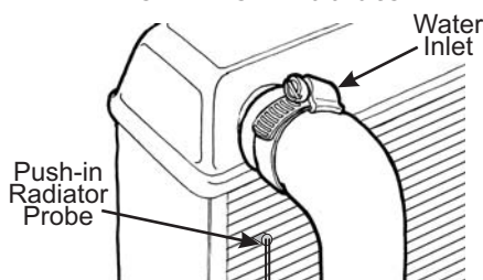
Down-flow Radiator
