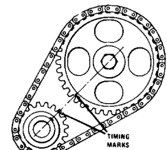
FORD 6-144, 170, 200, 250
