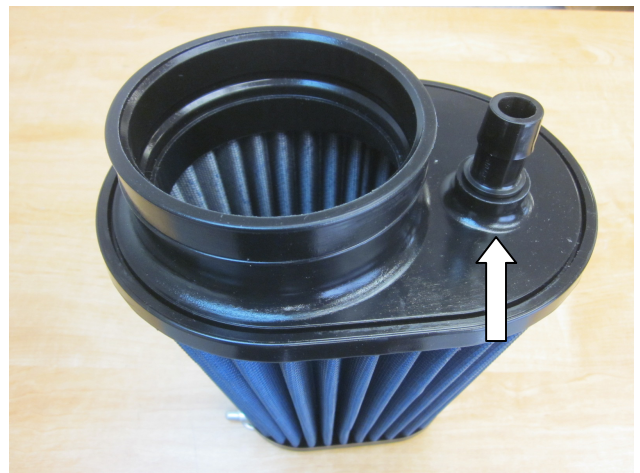
d) Install the supplied adaptor fitting into the hole on the Air Filter – the barbed end goes into the air filter.
