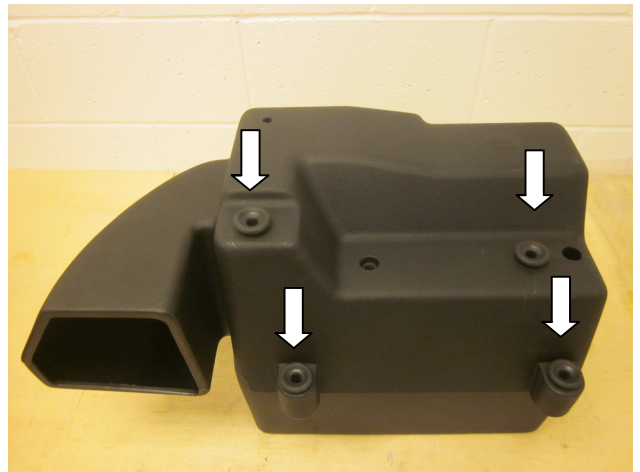
b) Insert the 4 rubber grommets removed in step 3a) into the bottom of the MOPAR Cold Air Box.
