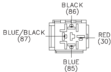
WIRE LOCATIONS (RELAY NOT SHOWN)
