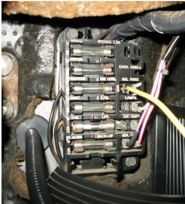
Figure 17 - Connect Power Wire
