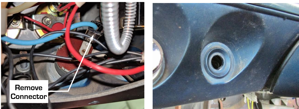
Figure 6 – Remove Factory Wiper Switch
