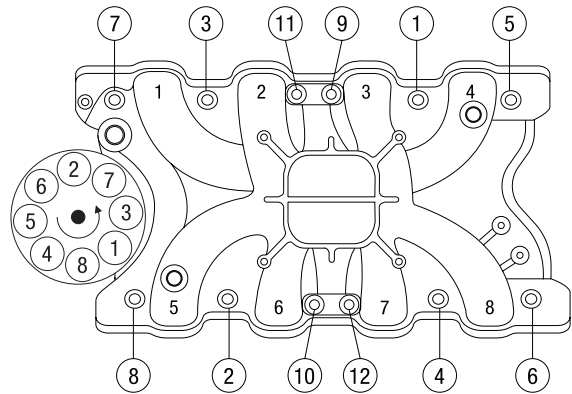
Figure 3 - 351-M/400 Ford Torque Sequence Torque Bolts to 25 ft/lbs. Firing Order: 1-3-7-2-6-5-4-8 Turn Distributor Clockwise to Advance Ignition Timing
