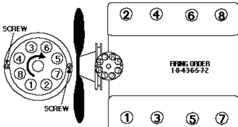
Figure 2- Rover 3.5 litre V-8 Turn distributor counter-clockwise to advance timing
