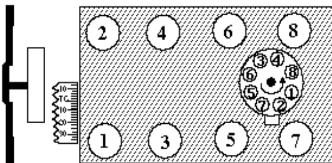
Figure 1- Pontiac 389-455 c.i.d. V8 Firing Order 1-8-4-3-6-5-7-2 Turn distributor clockwise to advance timing.
