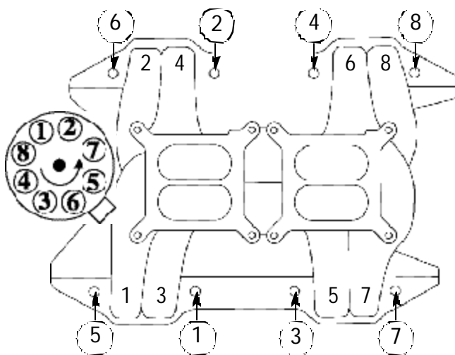
Figure 1 - 361-383-400 c.i.d. Chrysler Intake Manifold Torque Sequence
