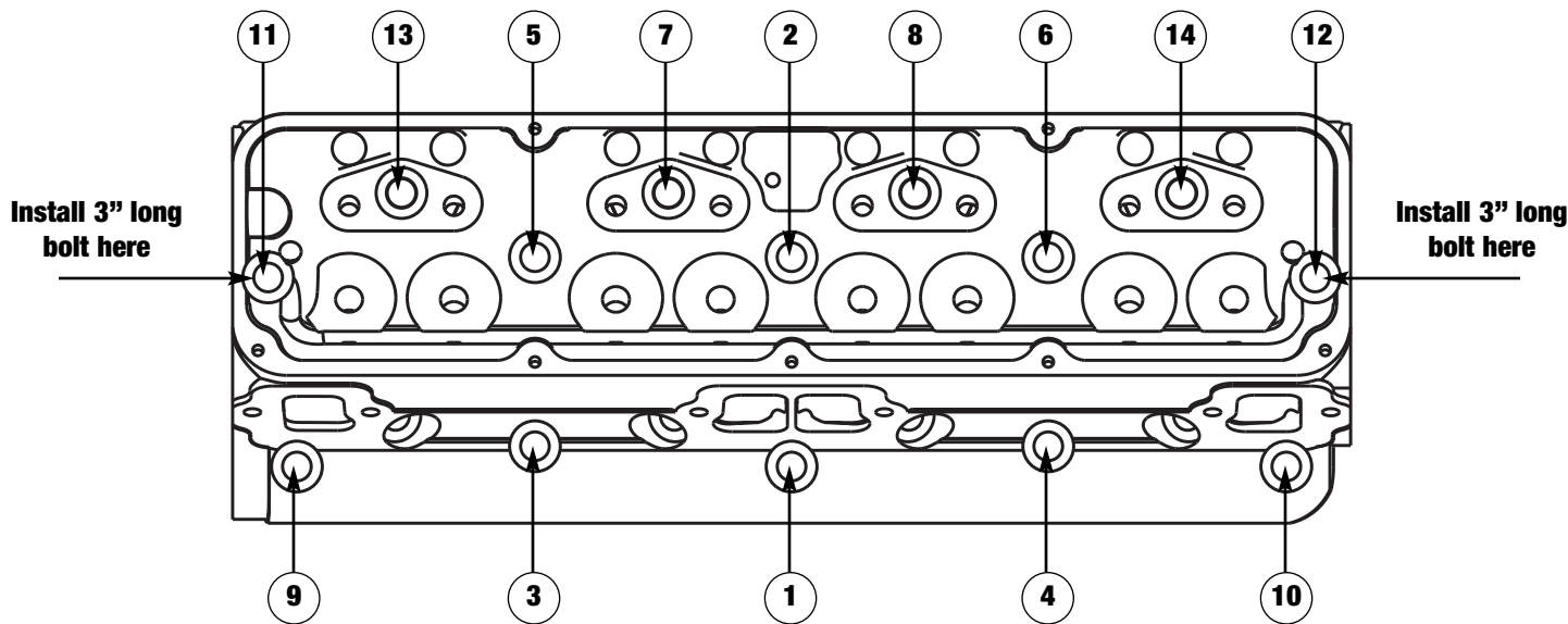
Figure 1 - AMC Cylinder Head Bolt Tightening Sequence (Tighten in four steps: 30, 40, 50, 65-70 or 30, 60, 90, 100-110 ft/lbs)
