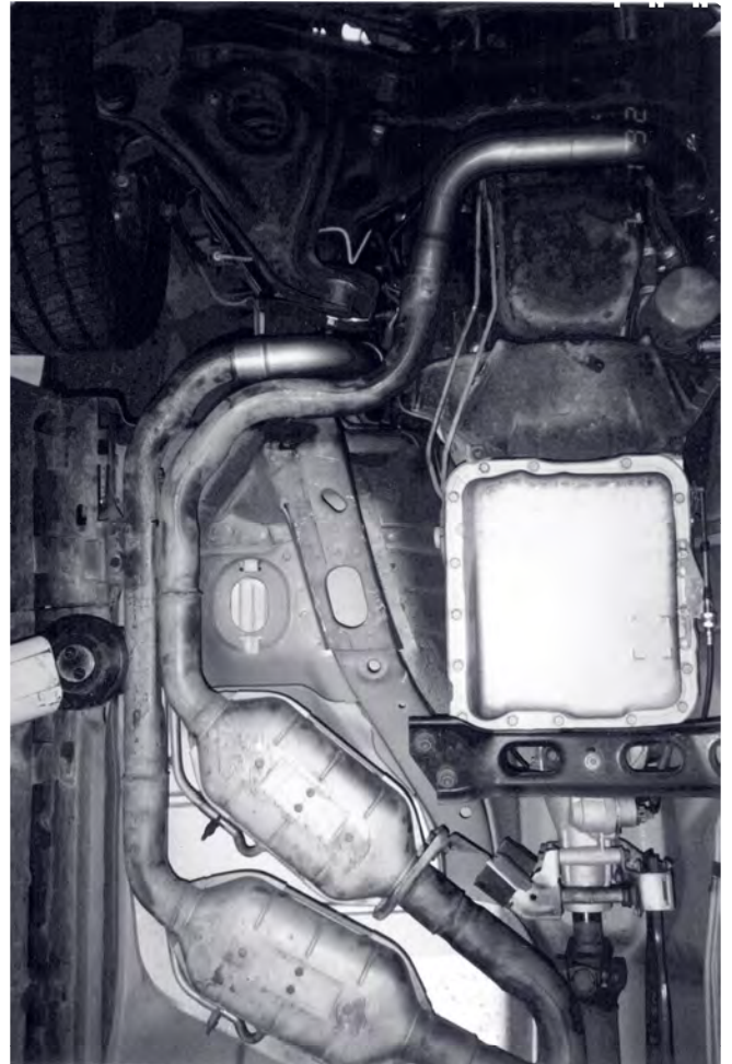
Figure 6 View from under vehicle of exhaust pipes/dual catalytic converter assembly after cutting and jointing to T.E.S.
