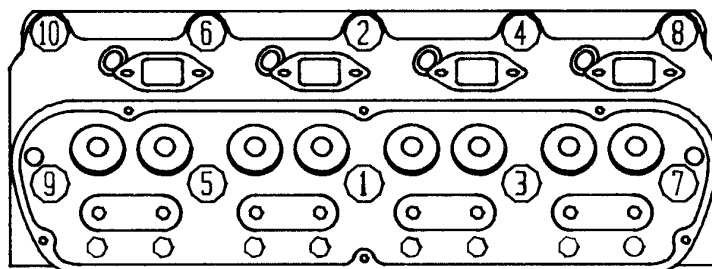
Figure 1 — Tightening Sequence
