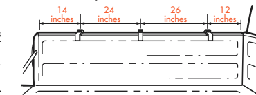
FORD FLARESIDE (3 clamps)
