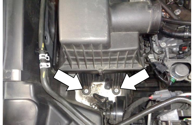
10. Remove the two airbox mounting nuts and retain for reinstallation at Step 18.
