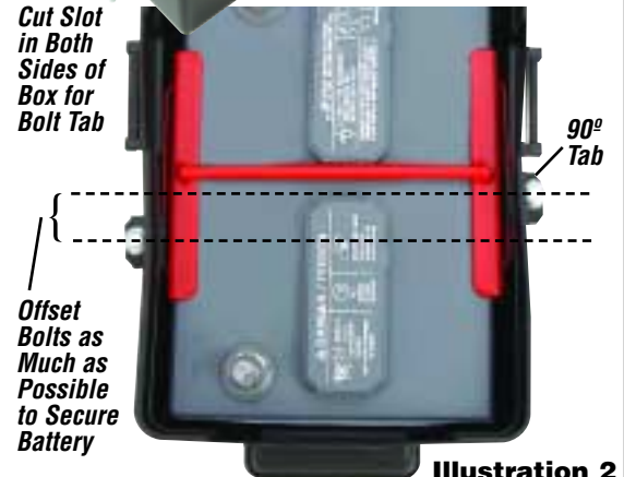
Illustration 2 Top View
