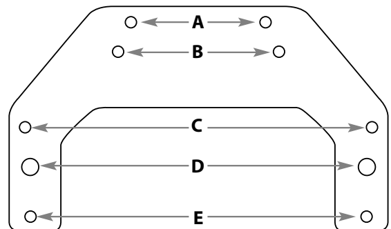
Turbo Adapter Plate
