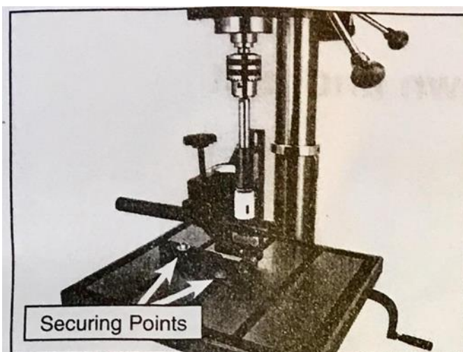
Figure 4. Mounting the jig to a drill press using a strap clamp in one location and a bolt with a t-nut in another location.
