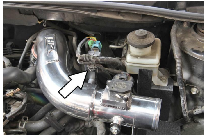
28. Clip the MAF sensor harness clip back onto the bracket.
