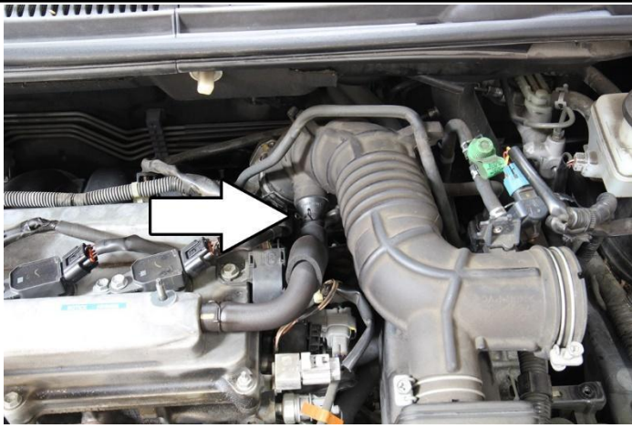
13. Disconnect the breather hose from the intake tube.
