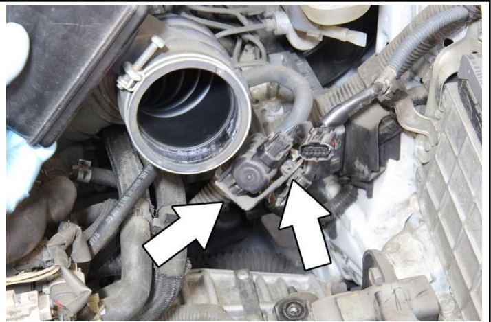
13. Remove the screw securing the EVAP sensor from the bracket, then depress the harness clip to remove to completely remove the electrical harness from the intake tube.
