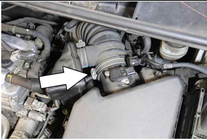
4. Loosen the hose clamp securing the factory intake tube from the air box assembly.
