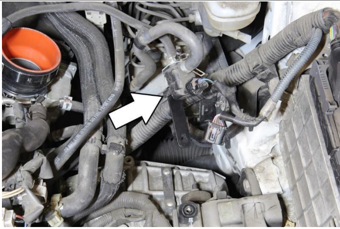
16. Install and secure the provided bracket onto the EVAP solenoid by using the factory screw and the M5 washer included in the hardware kit.
