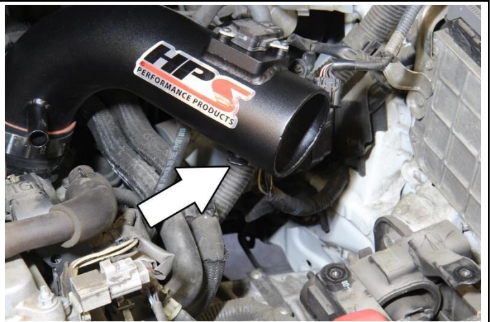
19. Secure the EVAP solenoid bracket to the intake pipe using the provided M6 x 12mm bolt and washer.
