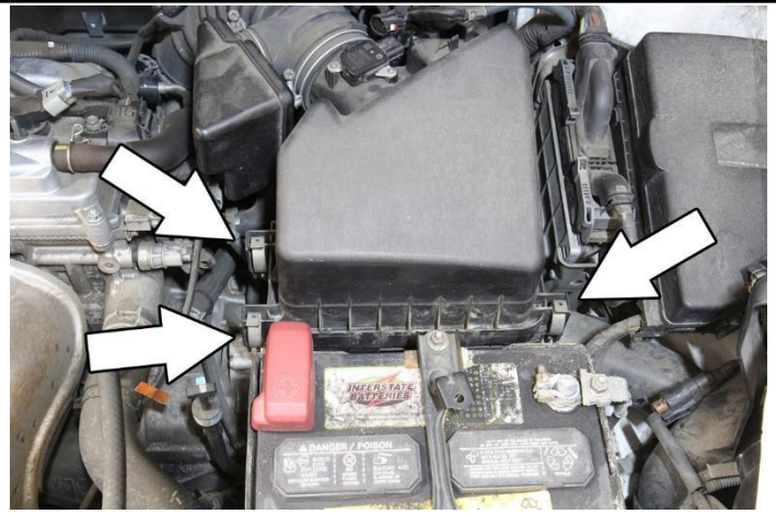
5. Disconnect the three retaining clips securing the upper air box assembly from the lower air box.
