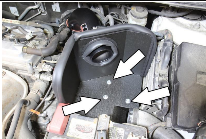
24. Insert the heat shield into the vehicle and secure the heat shield using the three M6 nuts and washers. Position the intake tube to the proper position and tighten the T-bolt clamp.
