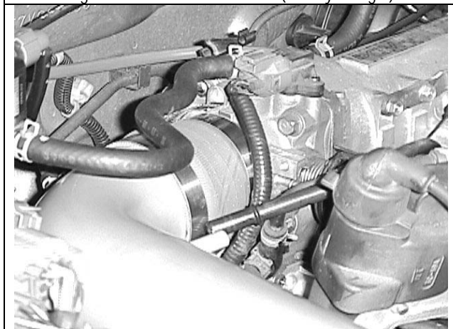
Fig 9: Connecting to throttle body. Note breather tube.
