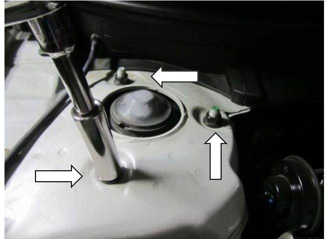
a. Remove the 3 Strut Tower nuts from each side needed to install the AEM Strut Tower bar.
