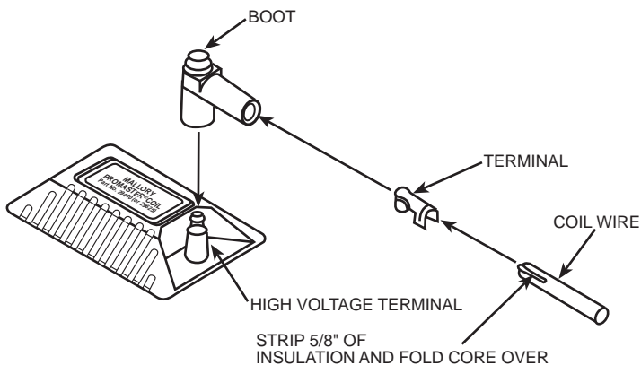
FIGURE 1A PROMASTER® IGNITION COIL
