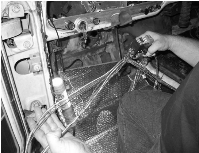
Figure 6-4 Routing Fuse Block to Base
