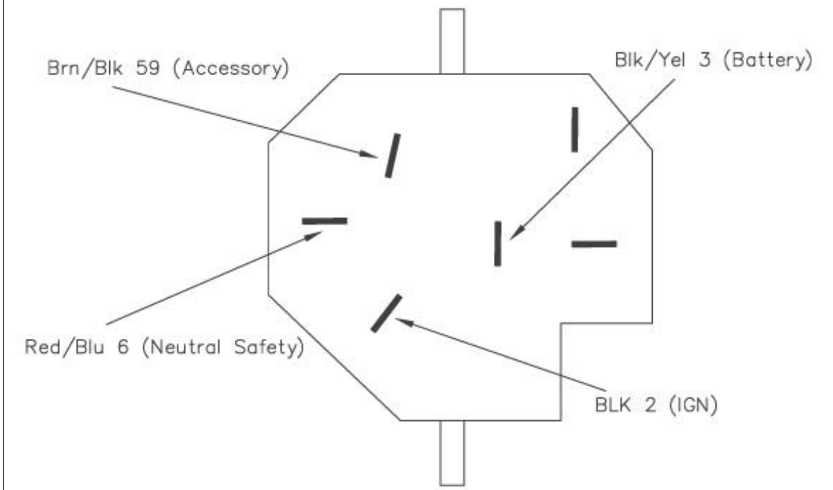
Figure 7-44 1977 Ford Truck Ignition Switch
