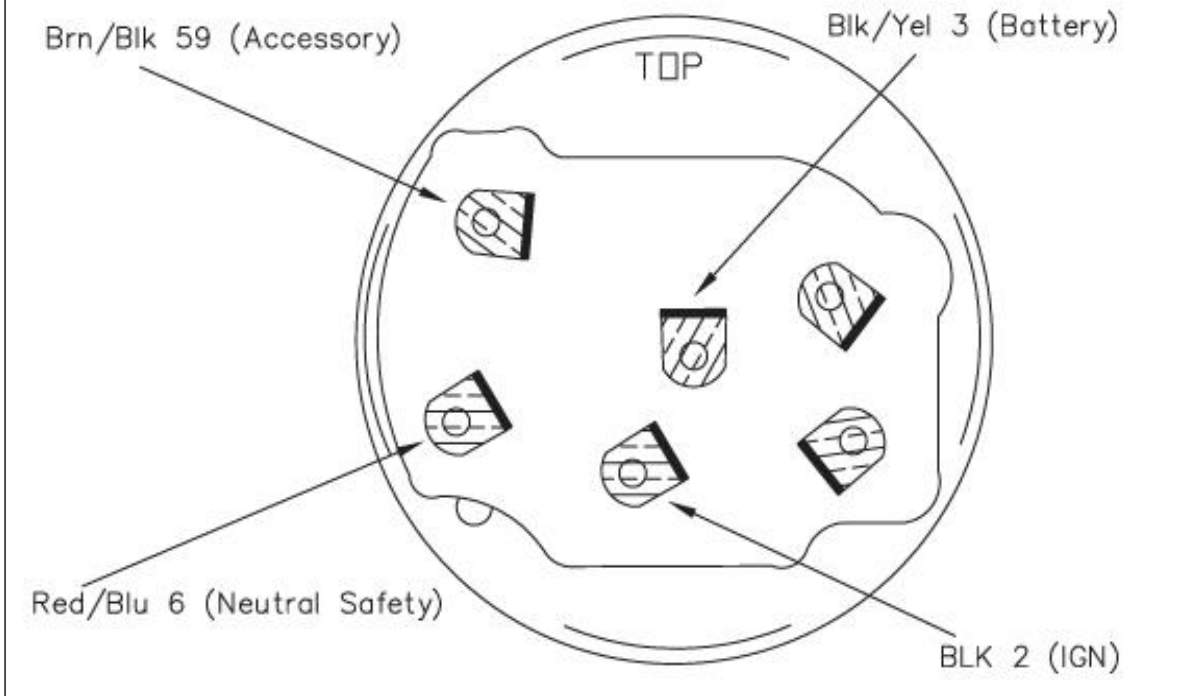
Figure 7-43 1970 – 1976 Ford Truck Ignition Switch
